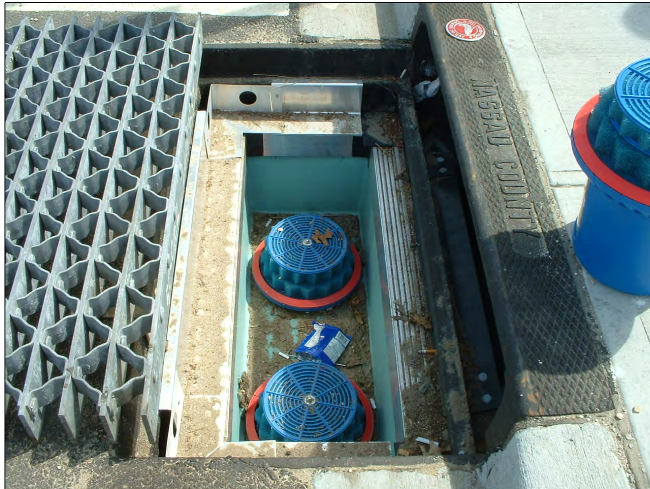
CATCH BASIN FILTER
